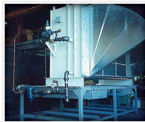
Make-Up Air Package with Posi-Pressure, Control System, and Rainhood
