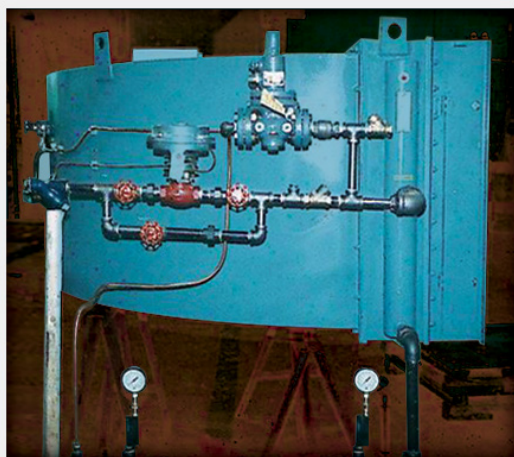
Posi-Pressure Control System Installed on a Make-Up Air Heater
