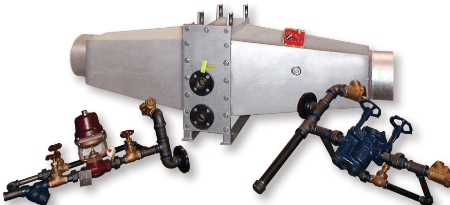
Extruder Air Heater Package with Transition Pieces, Steam Trap, and Control Valve
