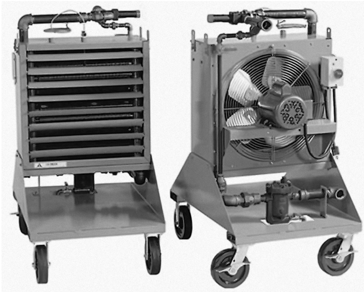
HotBreath™ Heater for Insect Pest Management or Temporary Heat
