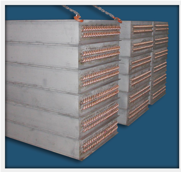
Duralite Plate Fin Coils (4 row full circuit)
